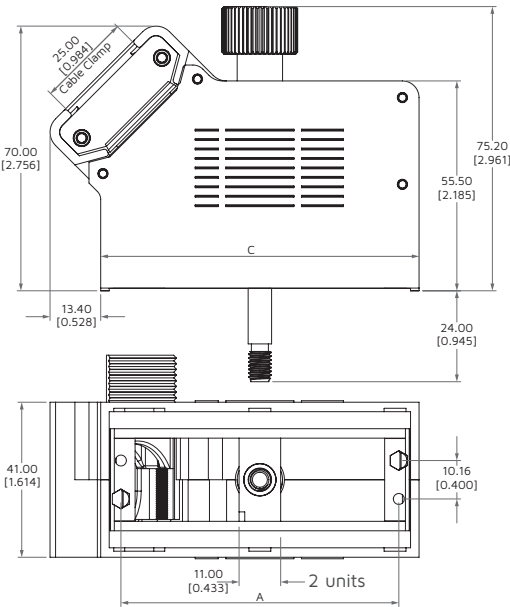
LEMVL Receptacle
