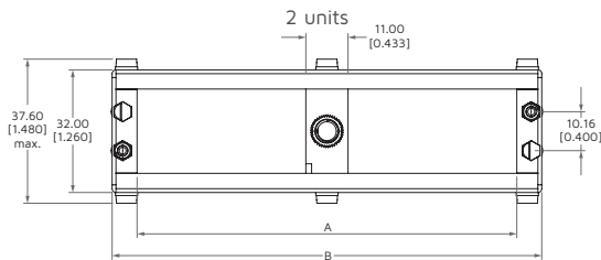
LEMVL Receptacle
