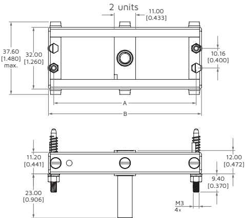
LEMVL Receptacle
